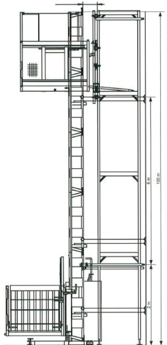
Tie spacing.
