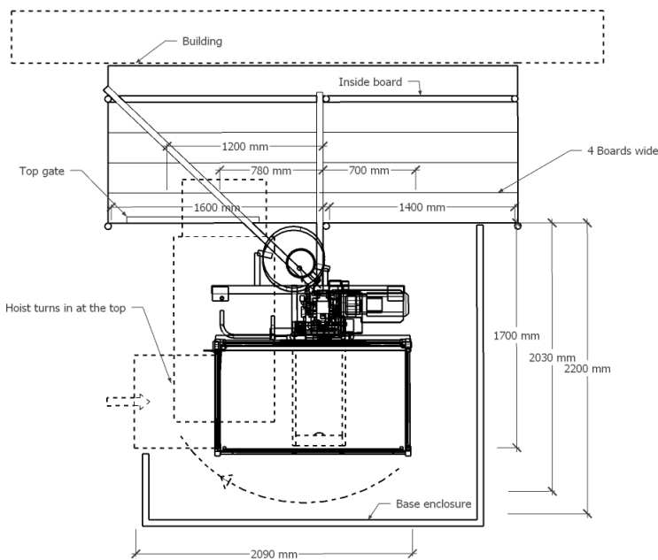
Scaffold installation.
