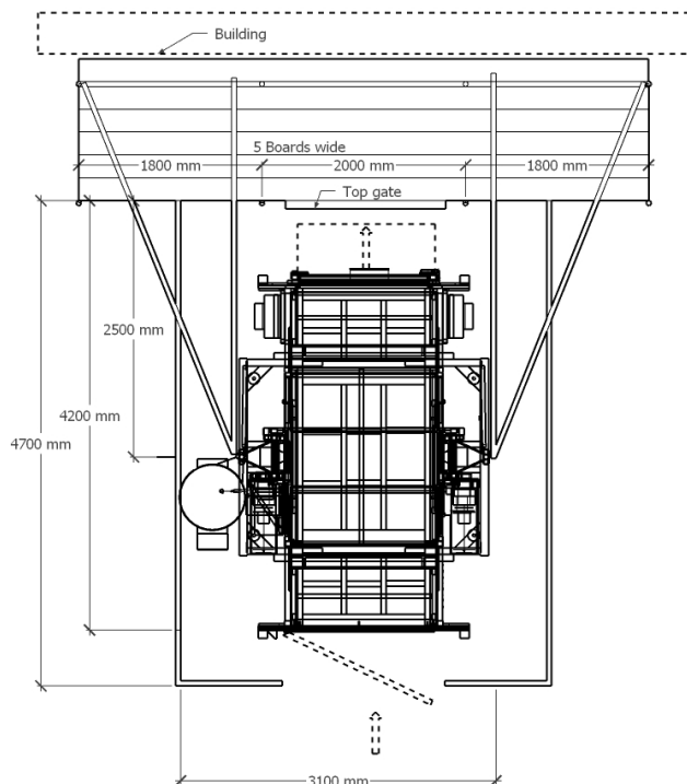
Space requirement for platform with base enclosure.
